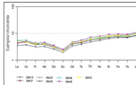
Fig. 6 Primitive Element-normalized multi-element diagram for Pyroxenites after Sun and McDonough (1989)
