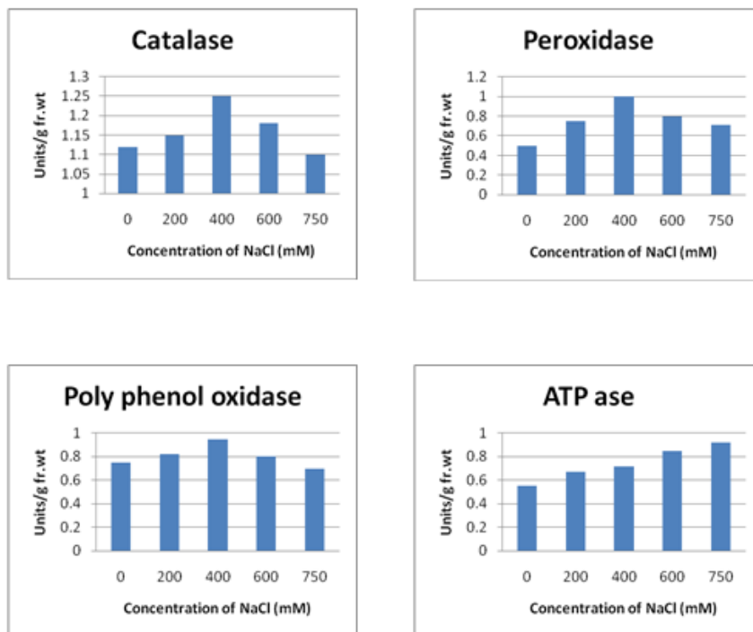
Fig I, Effect of NaCl on Catalase, Peroxidase, Polyphenol oxidase (Units \text{min}^{-1} \text{g}^{-1} \text{fr. wt} ) and ATPase (mM \text{No}_3 reduced \text{g}^{-1} \text{fr. wt h}^{-1} ) in the leaf of S. nudiflora
