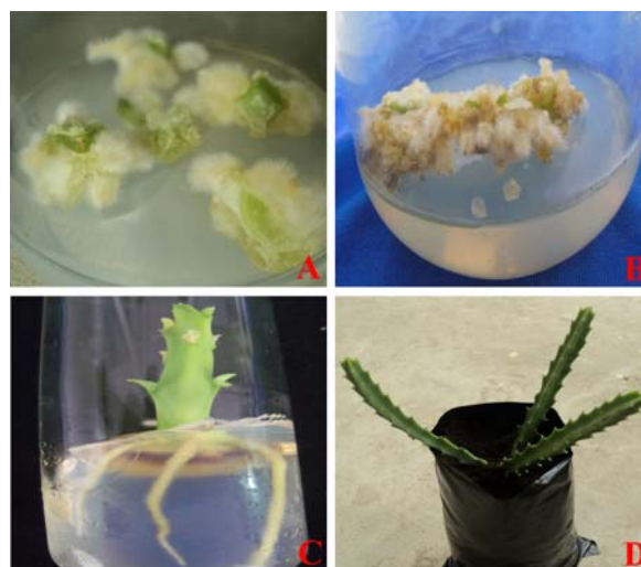
Figure. 2. (A and B) Induction of callus with rooting on regenerated shoots on half strength MS medium containing 2.0, 2.5\text{mg/L} of IBA + 0.5\text{mg/L} of NAA; (C) Extensive root growth on half strength MS medium containing 0.5\text{ mg/L} of IBA + 0.5\text{ mg/L} of NAA; (D) Acclimatized plantlet after four weeks.
