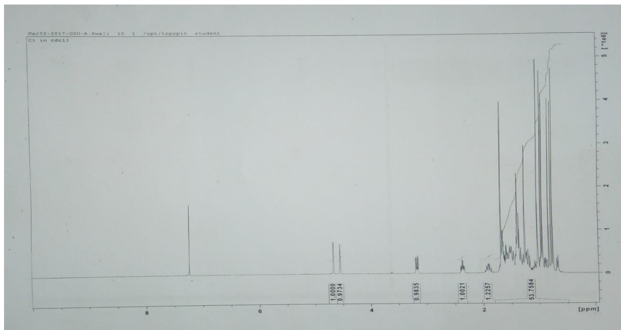
^1\text{H-NMR} spectrum of Enac1
